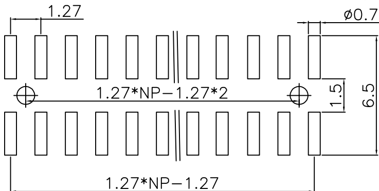
PCB LAYOUT
