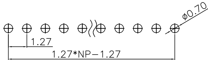
PCB LAYOUT
